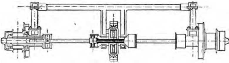
FIG. 35.—Jointed Rear-Axle of the DeDion & Bouton Carriages. By the use of universal joints between the driving spur and wheel spindles a steady drive may be maintained between the spur, hung on the body, above the springs, and the wheels, below the springs, even on the roughest roads, when the springs are constantly in action.
